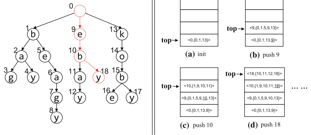
Fig. 12 Incremental similarity joins on sample data set in Fig. 2 ( \Delta S = \{\text{"eby"}\} , \tau = 1 )
