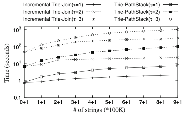
Fig. 29 Scalability on AOL Query Log (e.g., 6+1 denotes |S| = 600 K, |\Delta S| = 100 K)
