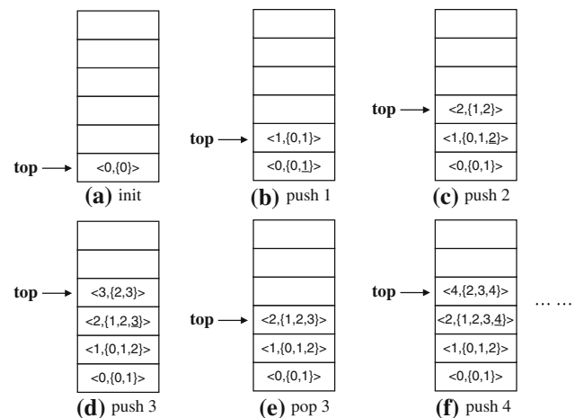
Fig. 9 An example to use TRIE-PATHSTACK algorithm to find all similar pairs ( \tau = 1 )
