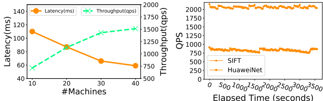
Figure 13: Scalability.
