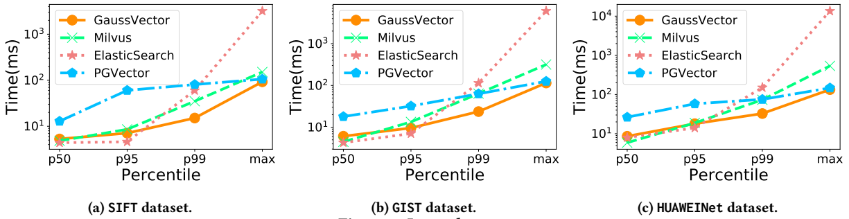
Figure 9: Insert latency.
